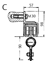
Sliding guide ways If required also available under lintel on 2 rails
