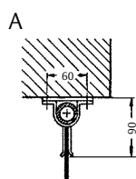
Ceiling fixing
