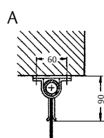
Ceiling fixing
